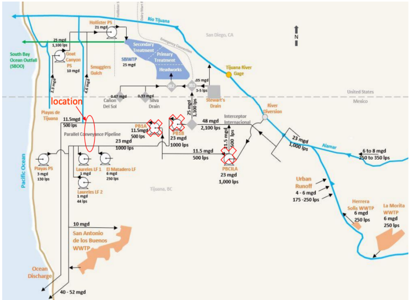
Figure 1. Minute 283 binational wastewater diversion and treatment system. 1
